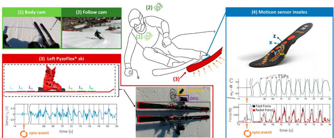
Figure 2. Experimental setup with: (1) body cam; (2) follow cam; (3) PyzoFlex ® ski prototype with data acquisition (DAQ) device, sync tool, and sensors L_1 to L_6 ; and (4) Moticon sensor insoles with the coordinate system ( x, y, z ) and the rotational velocity ( \omega_y ) around the y -axis for the roll angle ( RA ) calculation. The vertical gray lines in the diagrams correspond to the video-based turn switch points ( TSP ).
